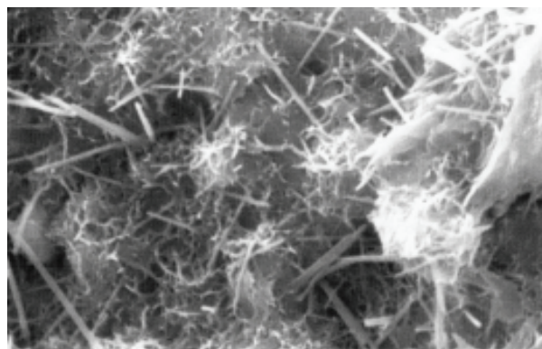
Fully developed crystal growth at 28 days within the capillary tracts of concrete blocking flow of water
